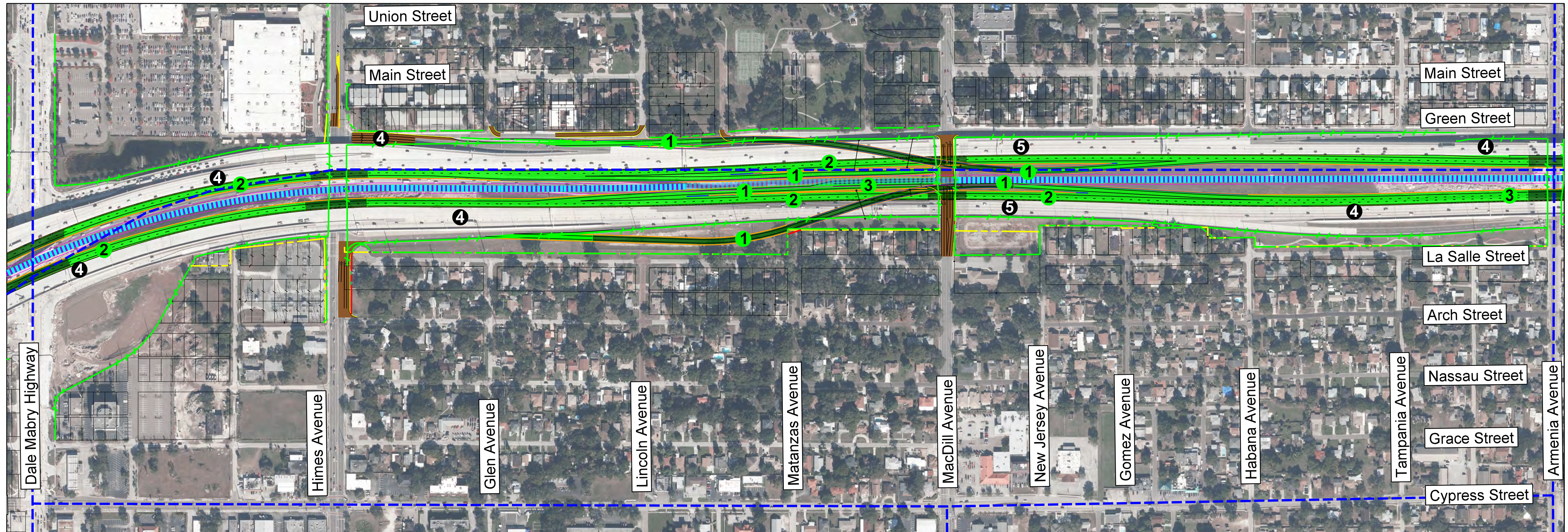
OPTION C - Express Lane Interchange South Side at MacDill Ave & North Side at Himes Ave (via fly-over ramps)
