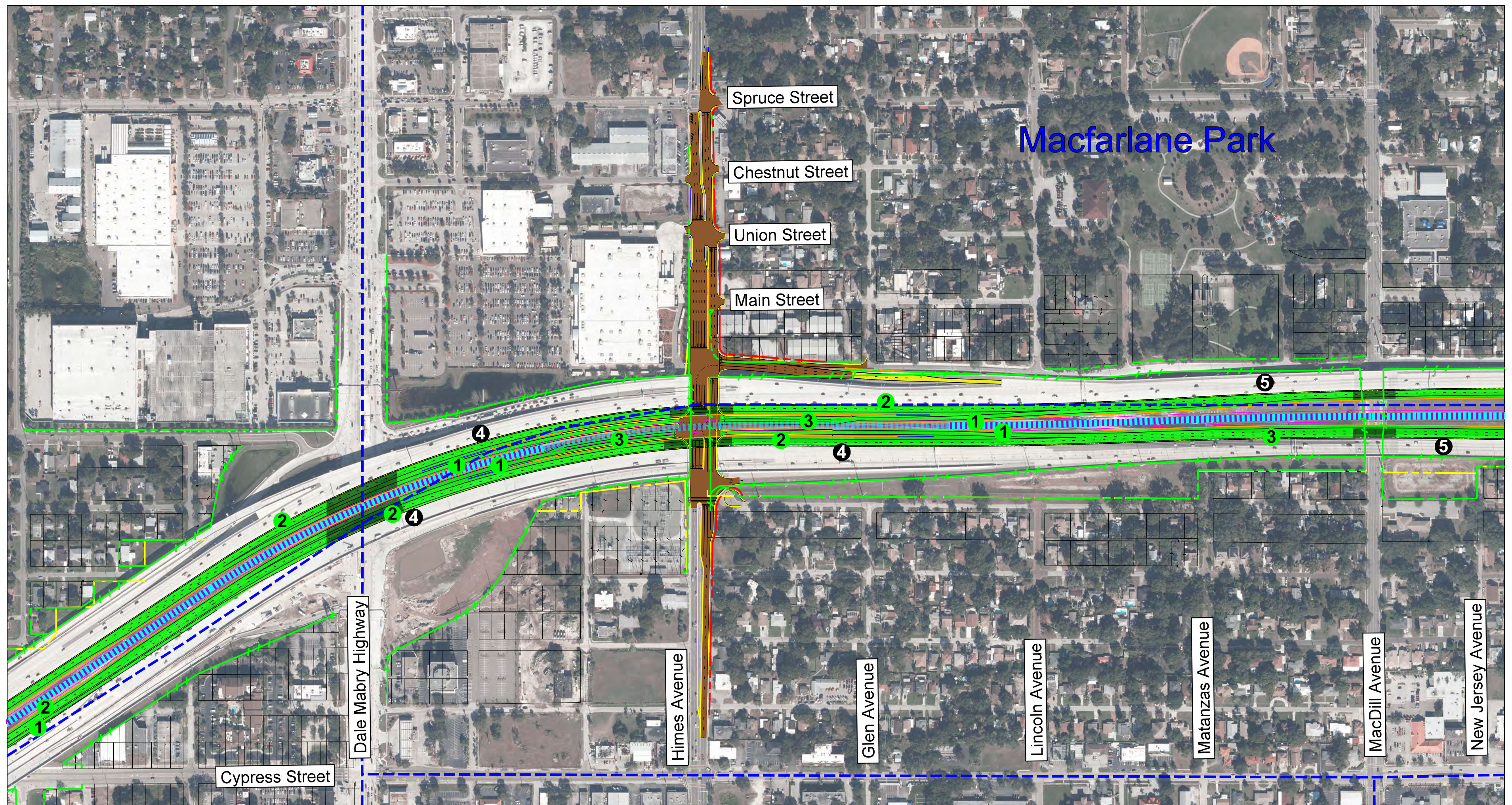
OPTION B - Full Express Lane Interchange at Himes Ave
